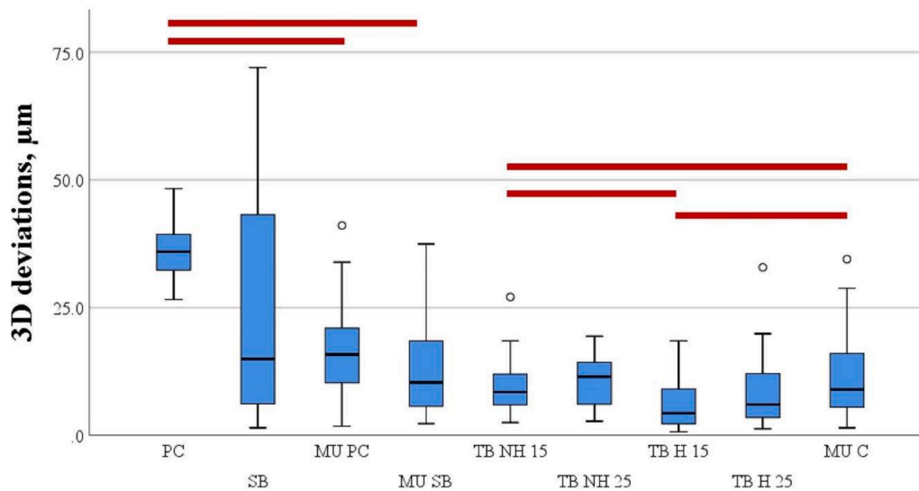
Fig. 4. Positional 3D deviations of tested components with statistically significant differences ( p < 0.05 ) between the groups marked with lines. (PC - Pick-up copings; SB - Scanbodies; MU PC - Multi-unit pick-up copings; MU SB - Multi-unit scanbodies; TB NH - Ti base non-hex, TB H - Ti base hex, MU C - Multi-unit caps.).
