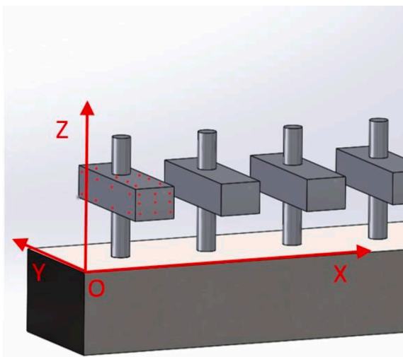
Fig. 1. Graphical representation of the steel block with an embedded dental implant and connected prosthetic component with attached gauge block. Red dots indicate the CMM measurement points.
